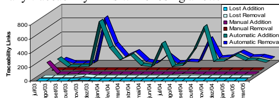
Figure 8: Traceability links evolution
