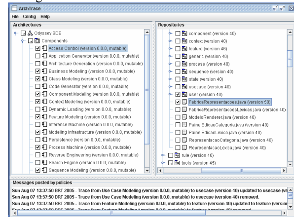
Figure 5: ArchTrace screenshot
